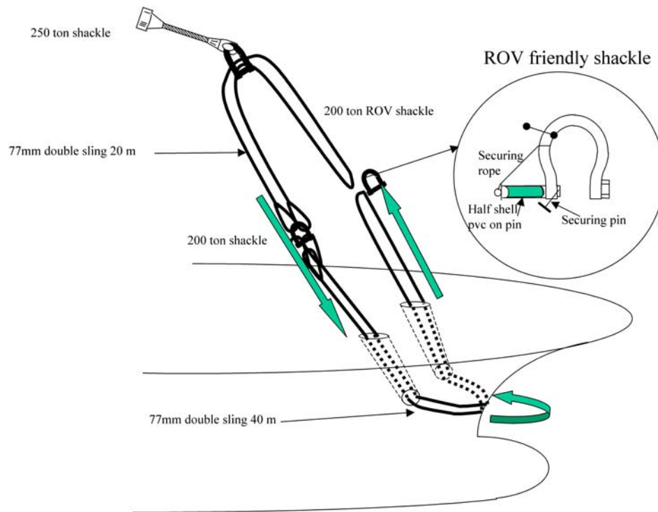
Figure 5-37. Concept to Lift Bow By Using the Hawse Pipes.
