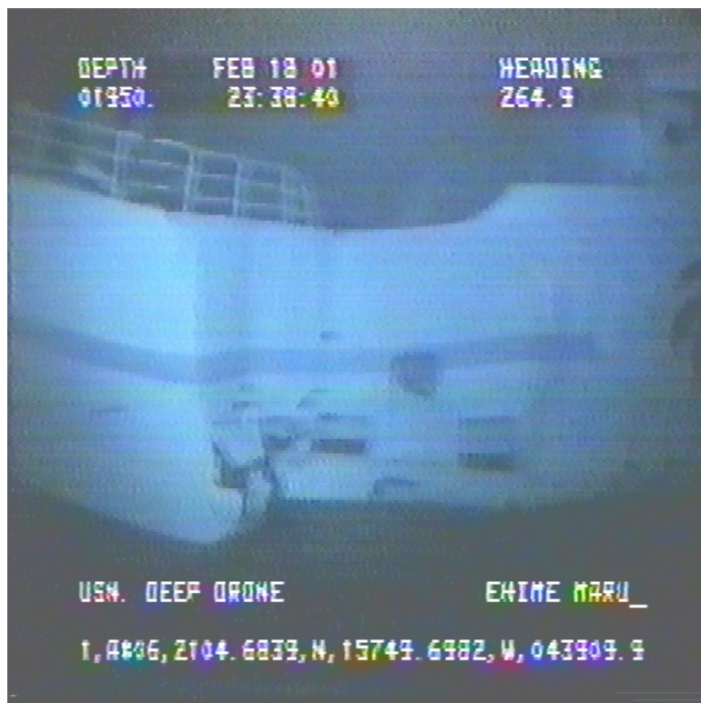
Figure 5-10. ROV Video Image of Port Side Forward Damage.
