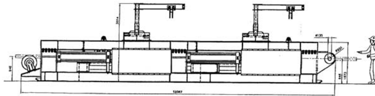
Linear Winch
