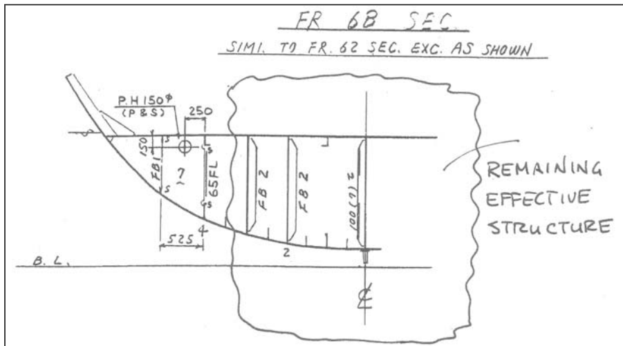
Figure 9. Station 7.5 (Frame 68) Section.
