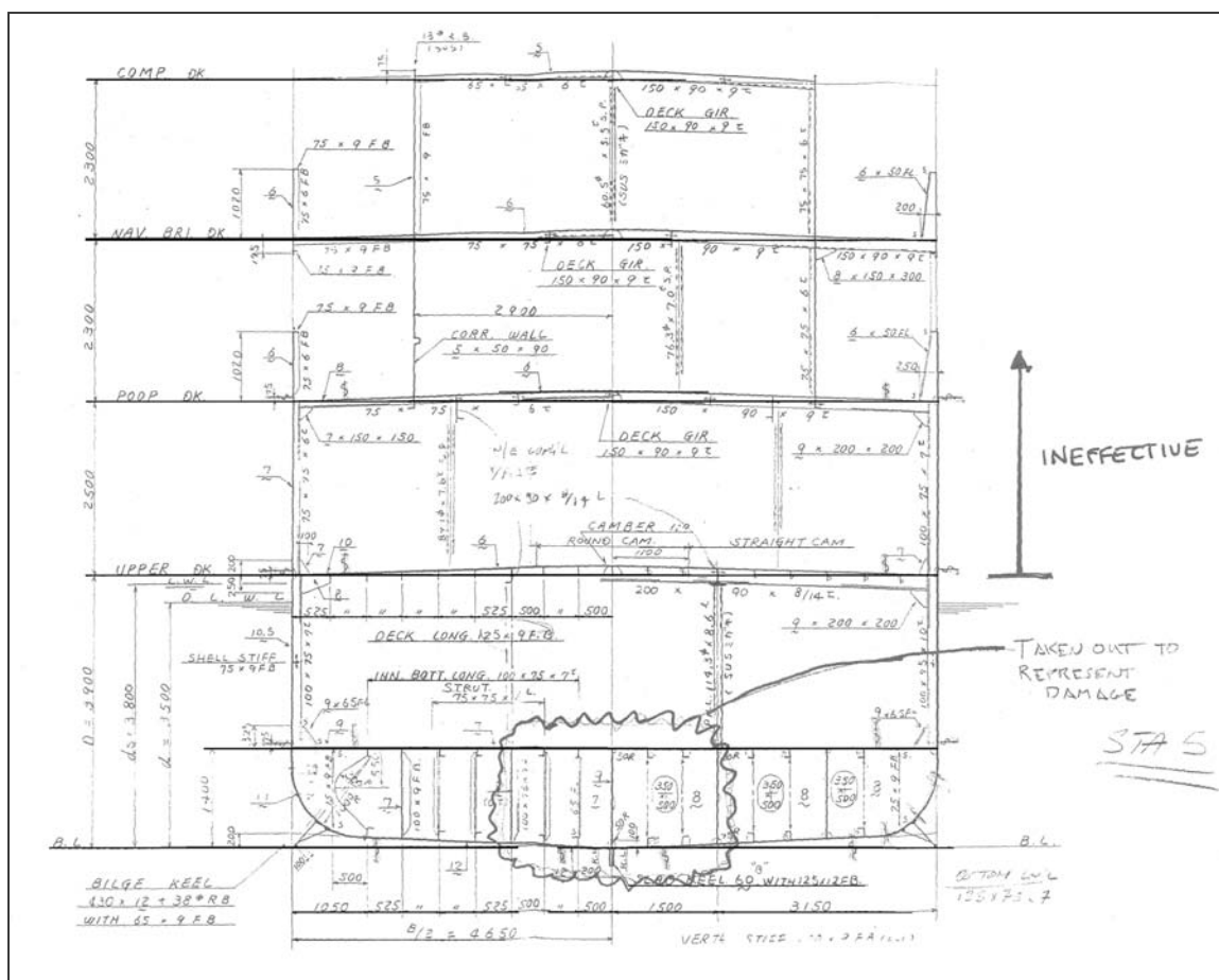
Figure 8. Station 4/5 (Midship) Section.
