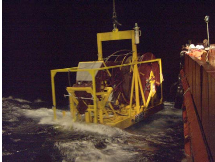
Figure 5-32. Launching Coiled-Tubing Drilling System.
